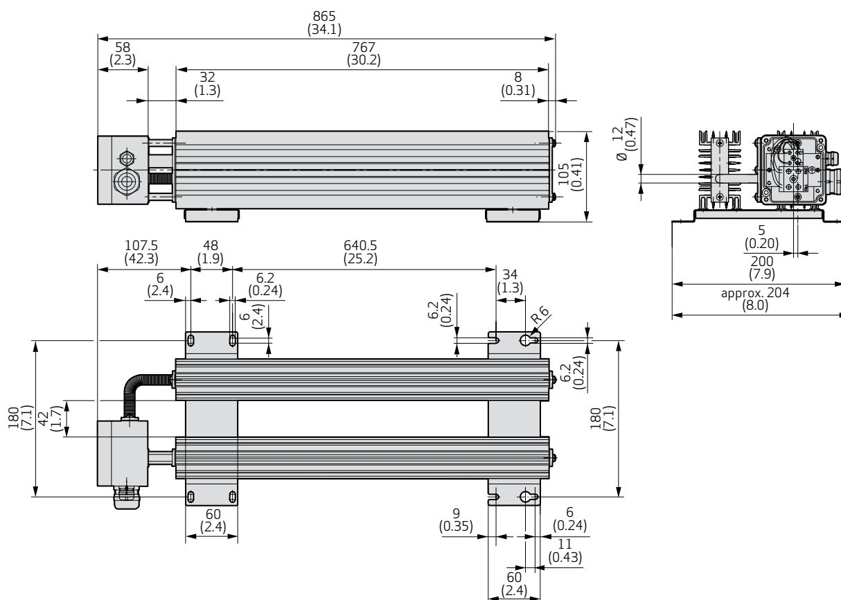
Dimensional drawing, braking resistor, A5
